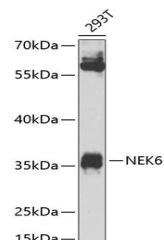
Western blot analysis of extracts of 293T...
