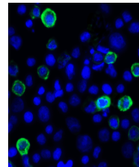
Immunofluorescence of LIGHT in transfect...
