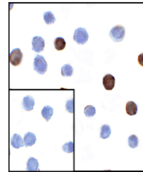
Immunocytochemistry of LIGHT in transfec...
