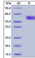
Human IL-1 RII, His Tag on SDS-PAGE unde...
