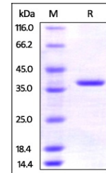
Human AIMP1, His Tag on SDS-PAGE under r...
