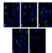
Immunofluorescence of VISTA in over expr...
