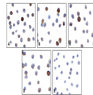
Immunocytochemistry of VISTA in over exp...
