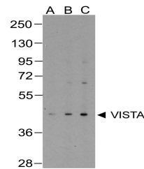
Western blot analysis of VISTA in over e...
