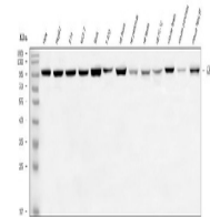
Western blot analysis of GRASP1/GRIPAP1
