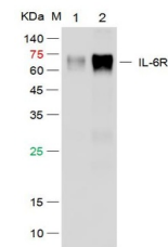
Western blot: Lane 1: Human IL-6R alpha Pr...
