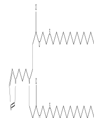
Chemical structure of orb1146681
