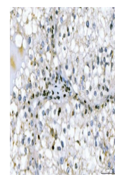
IHC analysis of GADD45B using anti-GADD45B antibody.
