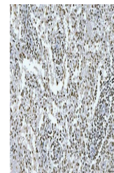
IHC analysis of GADD45B using anti-GADD45B antibody.
