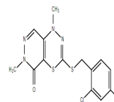
Chemical structure of GPR65 agonist (BTB...
