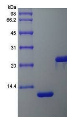
SDS-PAGE analysis of IL-5 protein
