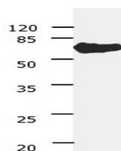
Western blot analysis of Gel: 10%SDS-PAG...
