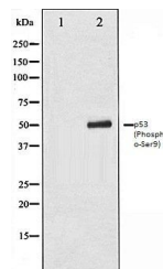
Western blot analysis of LOVO whole cell...
