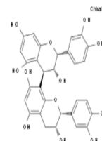
Chemical Structure: 29106-49-8
