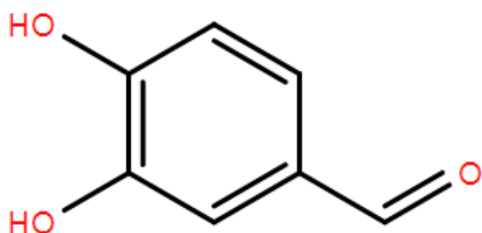
Chemical structure of Protocatechualdehyde.
