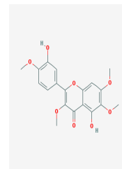
Chemical Structure of Casticin
