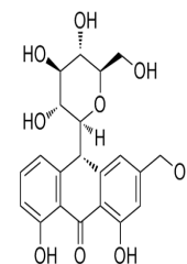
Chemical structure of Barbaloin.
