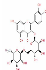
Chemical structure of Rutin
