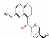
Chemical structure of Quinine
