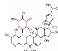
Chemical structure of Picfeltarraenin I A
