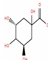
Chemical structure of Quinic acid
