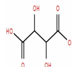
Chemical structure of D(-)-Tartaric acid
