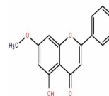
Chemical structure of 7-O- Methylchrysin
