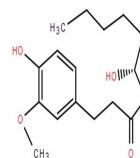
Chemical structure of 6-Gingerol
