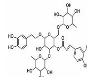
Chemical structure of Poliumoside
