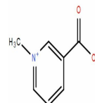
Chemical structure of Trigonelline
