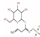
Chemical structure of Sinigrin
