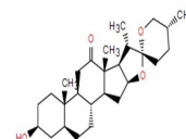
Chemical structure of Hecogenin
