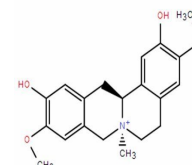
Chemical structure of Phellodendrine
