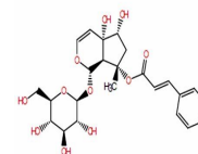
Chemical structure of Harpagoside
