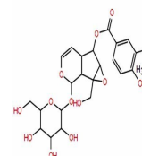
Chemical structure of Picroside II
