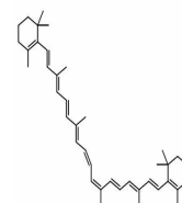
Chemical structure of beta-Carotene
