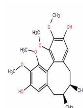
Chemical structure of Gomisin J
