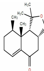
Chemical structure of Nardosinone
