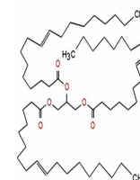
Chemical structure of Triolein
