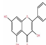
Chemical structure of 3
