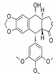
Chemical structure of Podophyllotoxin
