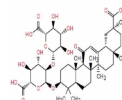
Chemical structure of Glycyrrhizic acid
