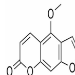
Chemical structure of Bergapten
