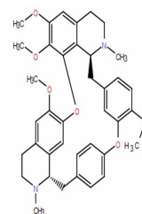
Chemical structure of Tetrandrine
