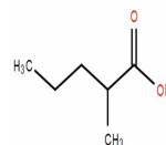
Chemical structure of 2-Methylvaleric ac...
