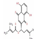
Chemical structure of beta
