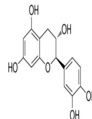
Chemical structure of Cianidanol.
