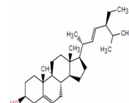
Chemical structure of Stigmasterol
