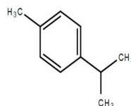
Chemical structure of 4-Isopropyltoluene
