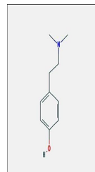
Chemical structure of Hordeanine
