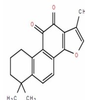
Chemical structure of Tanshinone IIA
