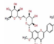
Chemical structure of pectolarin
