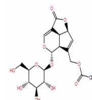
Chemical structure of Asperuloside
