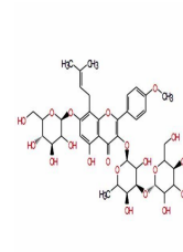
Chemical structure of Epimedin A1
